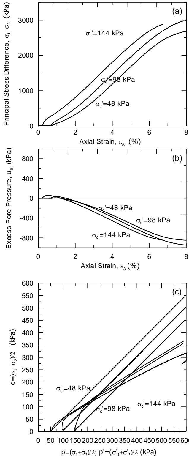
Figure 6.7. Static Triaxial Test Results for D6-Dorchester-03; B-1: a) Principal Stress Difference versus Axial Strain, b) Excess Pore Pressure versus Axial Strain, and c) Effective and Total Stress Paths.
