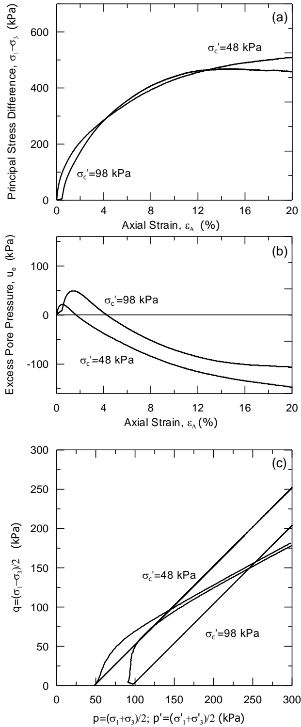
Figure 6.4. Static Triaxial Test Results for D1-Lexington-05; B-1: a) Principal Stress Difference versus Axial Strain, b) Excess Pore Pressure versus Axial Strain, and c) Effective and Total Stress Paths.
