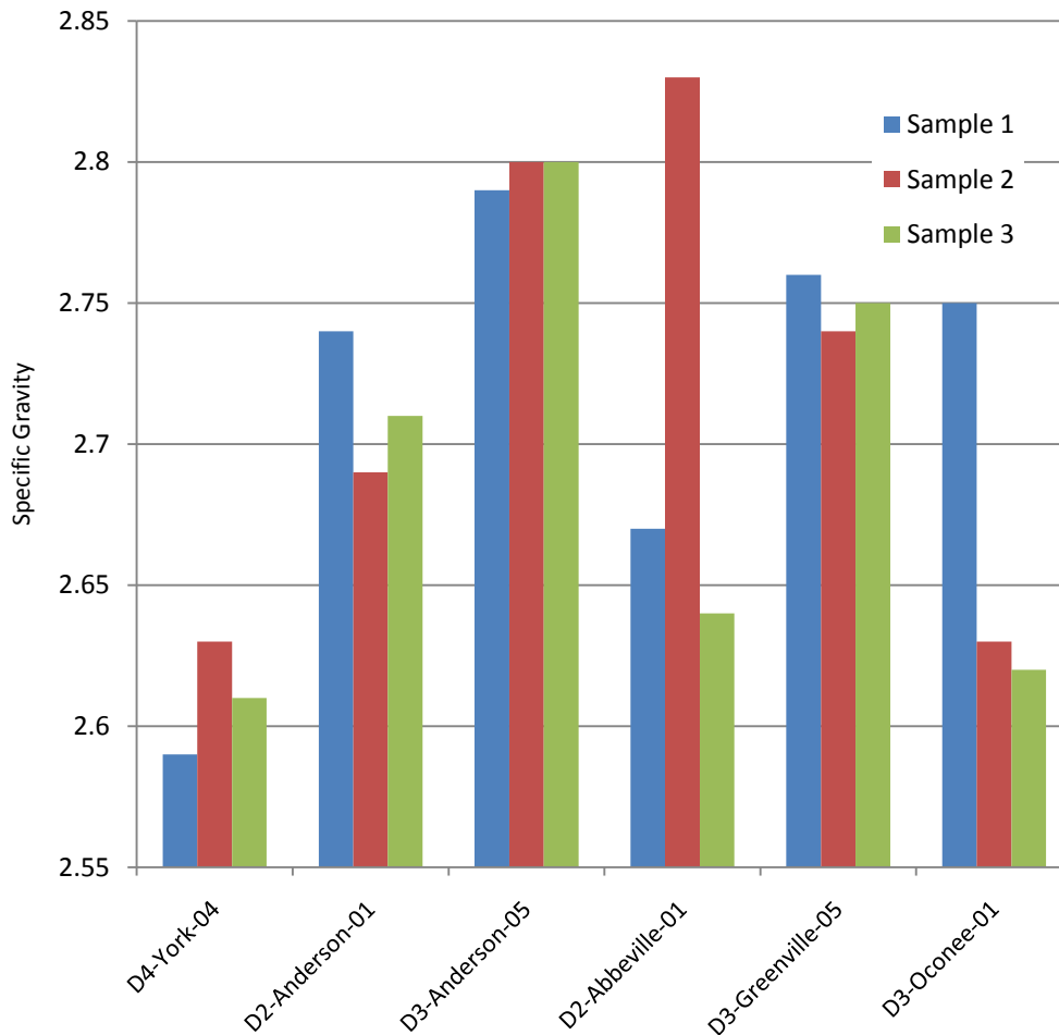
Figure 5.1. Specific Gravity, G_s , of Group A Soils
