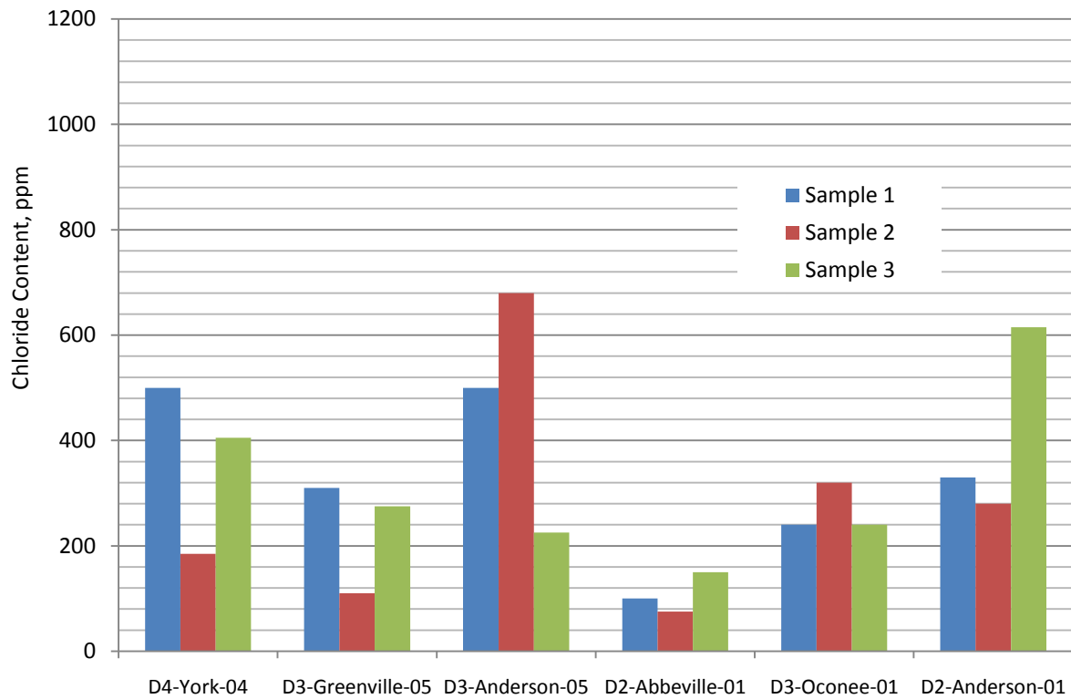
Figure 5.11. Chloride Content for Group A Soils
