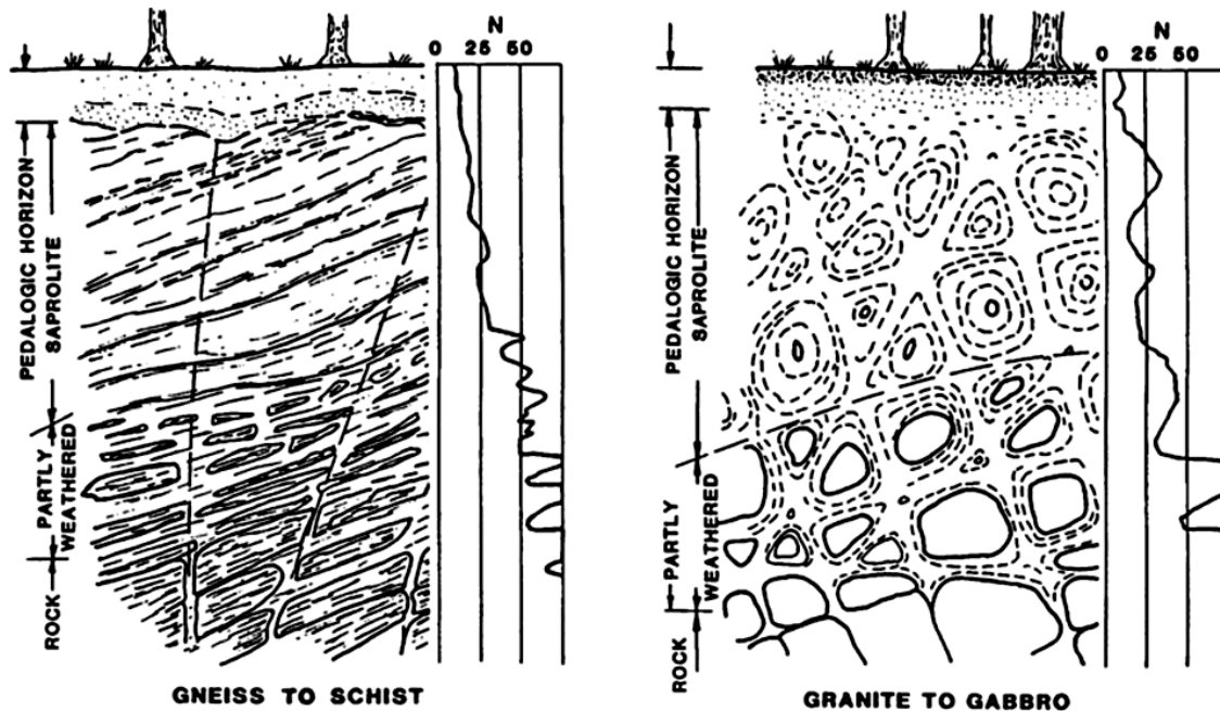
Figure 2.6. Piedmont Weathering Profiles (Sowers 1994)
