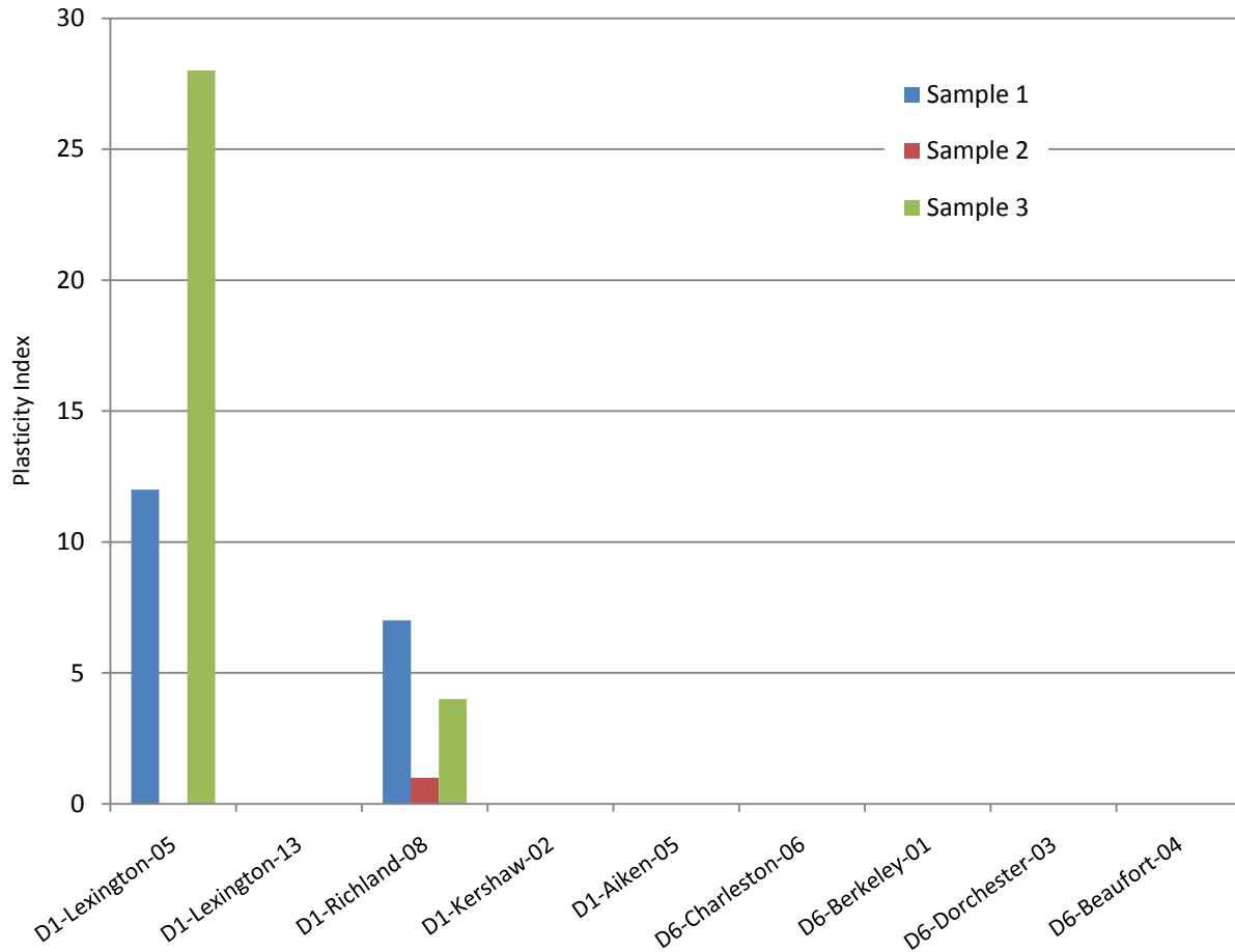
Figure 5.4. Plasticity Index, PI, of Group B Soils
