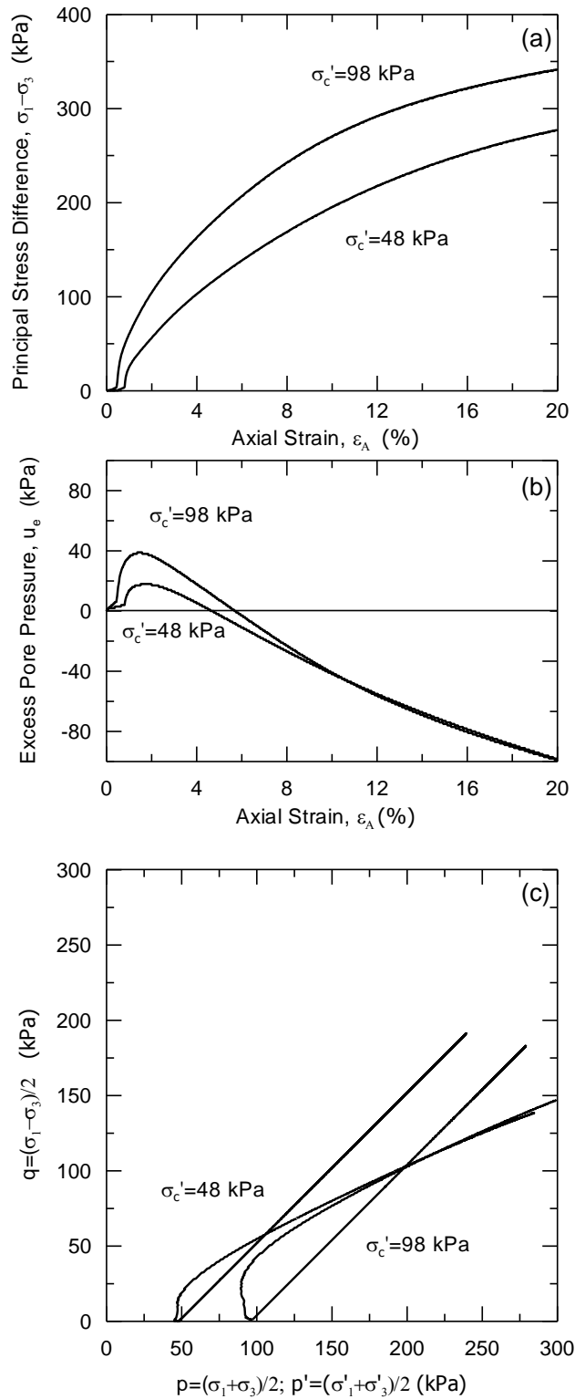
Figure 6.5. Static Triaxial Test Results for D1-Richland-08; B-1: a) Principal Stress Difference versus Axial Strain, b) Excess Pore Pressure versus Axial Strain, and c) Effective and Total Stress Paths.
