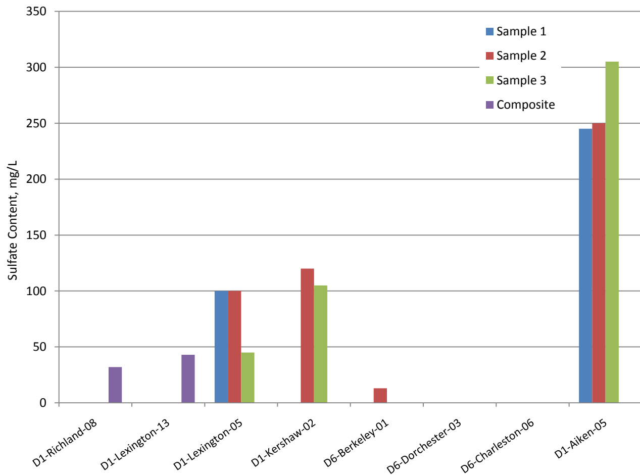
Figure 5.14. Sulfate Content for Group B Soils
