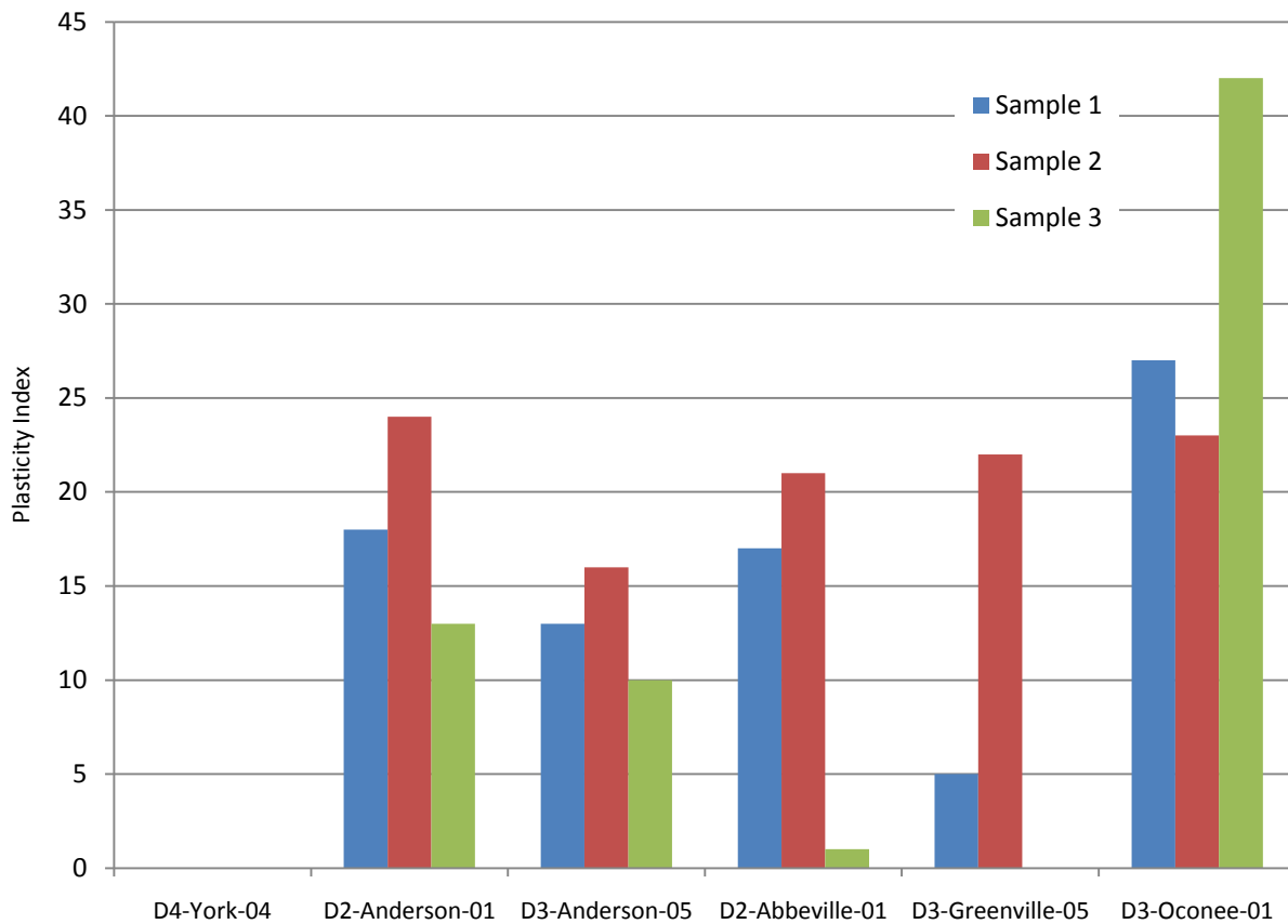
Figure 5.3. Plasticity Index, PI, of Group A Soils
