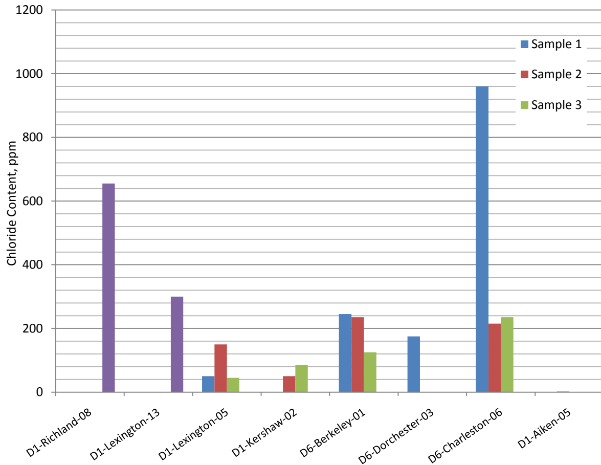
Figure 5.12. Chloride Content for Group B Soils
