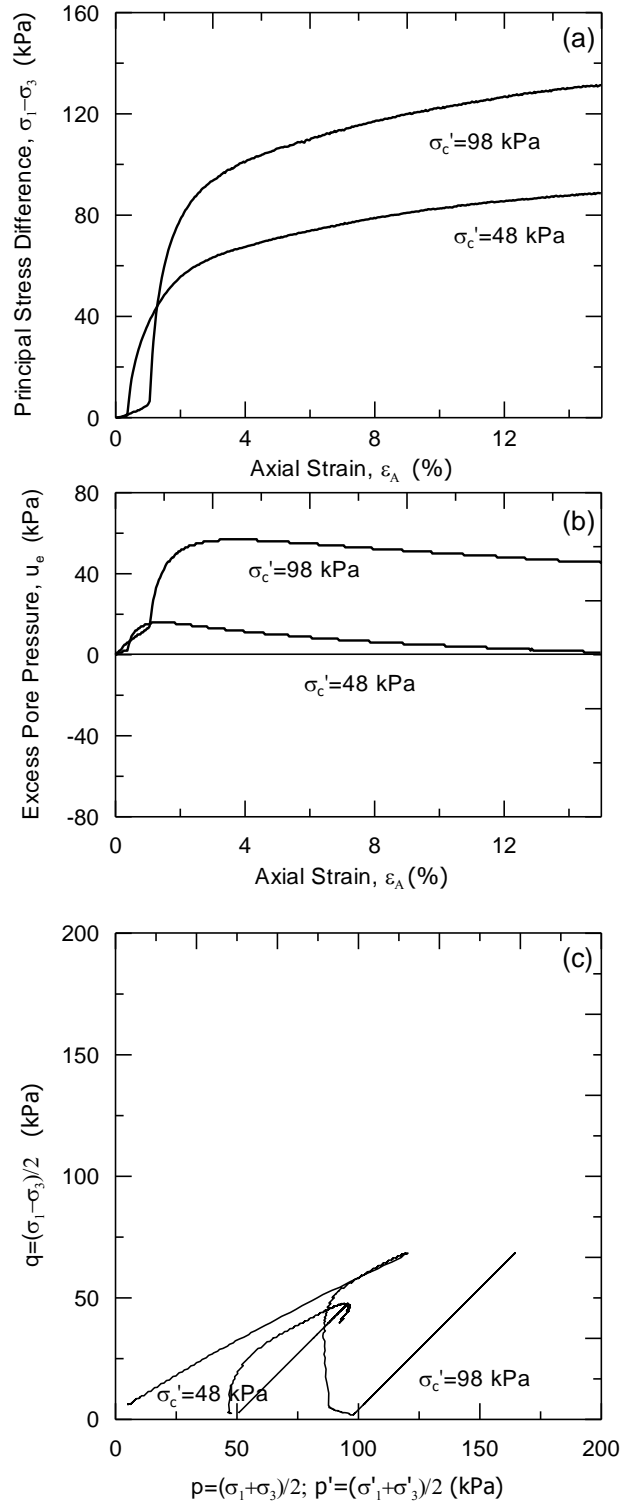
Figure 6.8. Static Triaxial Test Results for D2-Abbeville-01; B-1: a) Principal Stress Difference versus Axial Strain, b) Excess Pore Pressure versus Axial Strain, and c) Effective and Total Stress Paths.
