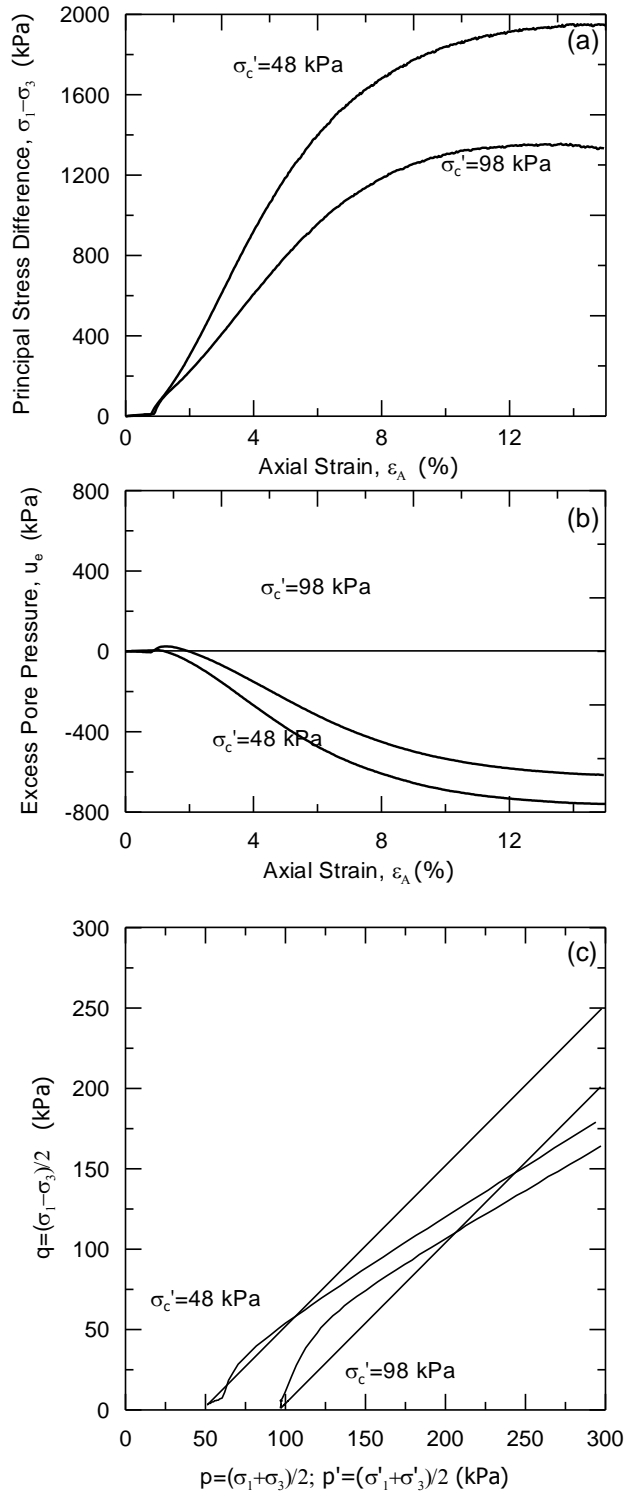
Figure 6.9. Static Triaxial Test Results for Charleston; B-1: a) Principal Stress Difference versus Axial Strain, b) Excess Pore Pressure versus Axial Strain, and c) Effective and Total Stress Paths.
