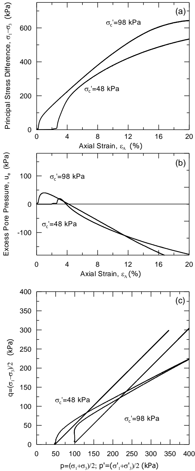
Figure 6.6. Static Triaxial Test Results for D6-Berkely-01; B-2: a) Principal Stress Difference versus Axial Strain, b) Excess Pore Pressure versus Axial Strain, and c) Effective and Total Stress Paths.
