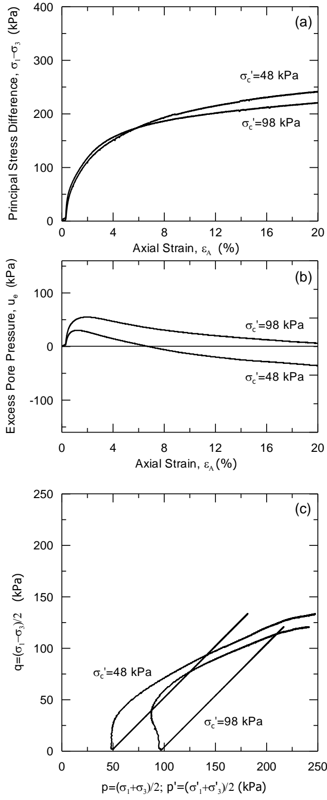
Figure 6.3. Static Triaxial Test Results for D2-Anderson-01; B-1: a) Principal Stress Difference versus Axial Strain, b) Excess Pore Pressure versus Axial Strain, and c) Effective and Total Stress Paths.
