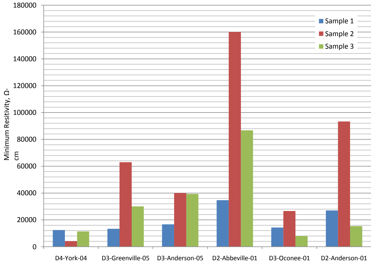
Figure 5.9. Soil Resistivity for Group A Soils
