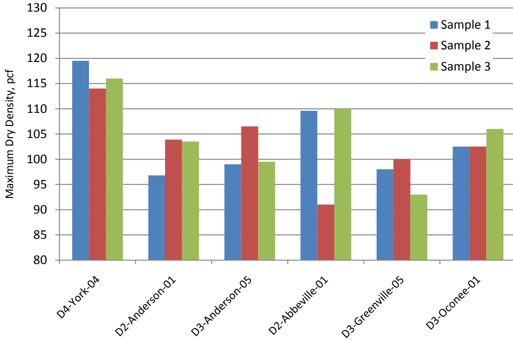
Figure 5.5. Maximum Dry Density of Group A Soils
