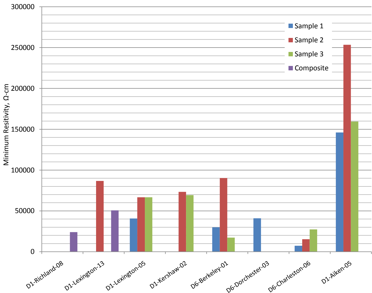
Figure 5.10. Soil Resistivity for Group B Soils
