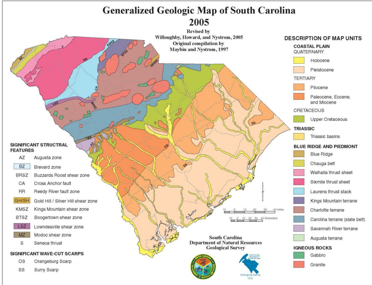
Figure 2.4. Generalized Geologic Map of South Carolina (South Carolina Department of Natural Resources, http://www.dnr.sc.gov/geology/geology.htm )
