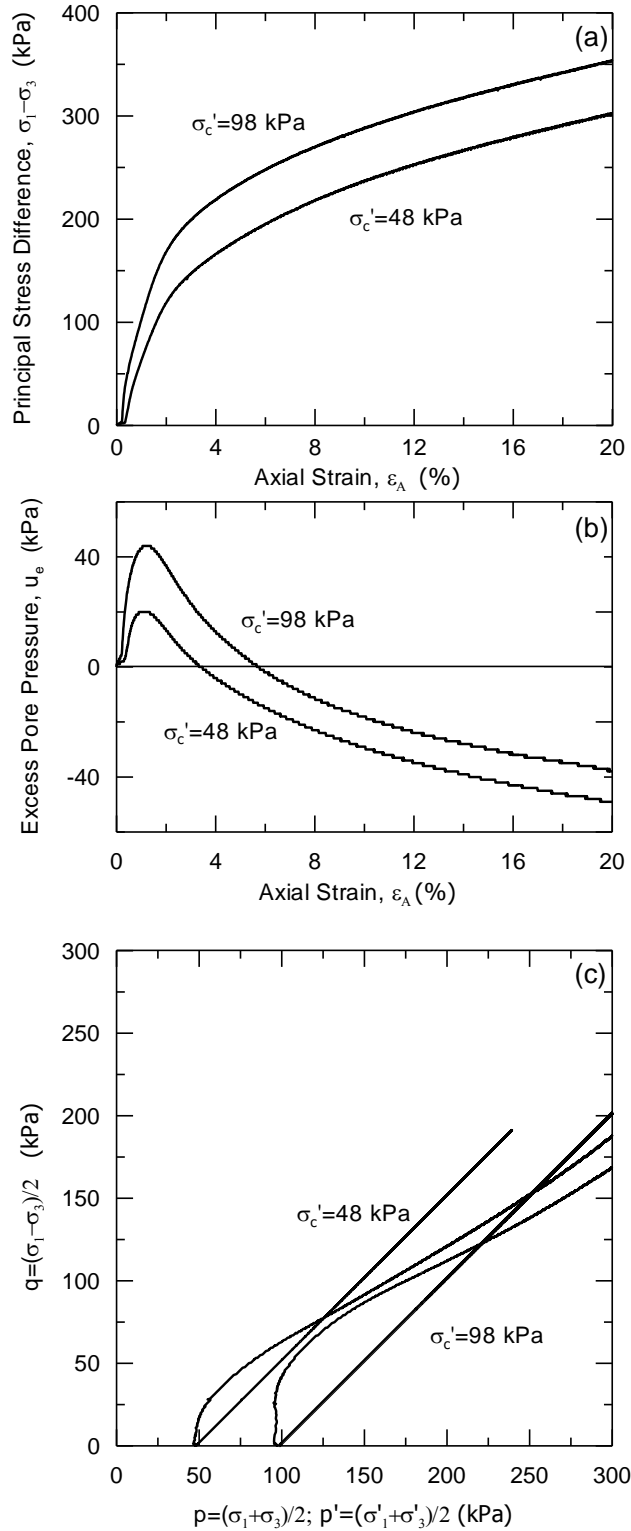
Figure 6.2. Static Triaxial Test Results for D4-York-04; B-2: a) Principal Stress Difference versus Axial Strain, b) Excess Pore Pressure versus Axial Strain, and c) Effective and Total Stress Paths.
