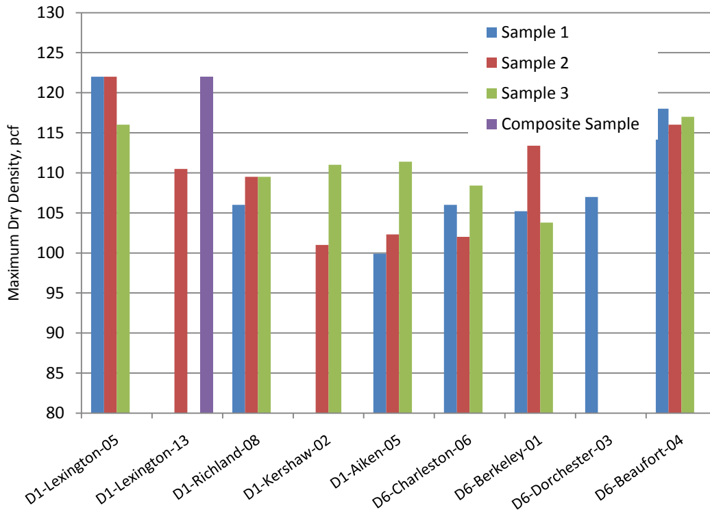
Figure 5.6. Maximum Dry Density of Group B Soils
