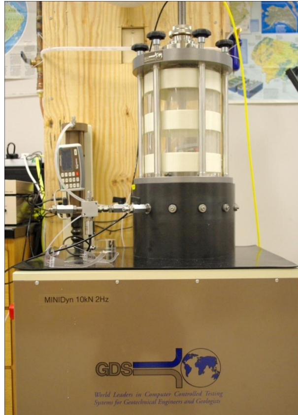
Figure 4.1. GDS Electromechanical Dynamic Triaxial Testing System (DYNTTS) in the Department of Civil and Environmental Engineering Advanced Geotechnical Laboratory.
