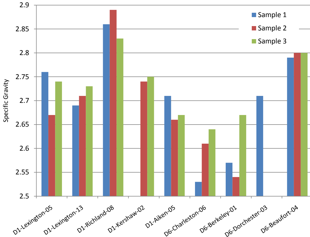
Figure 5.2. Specific Gravity, G_s , of Group B Soils
