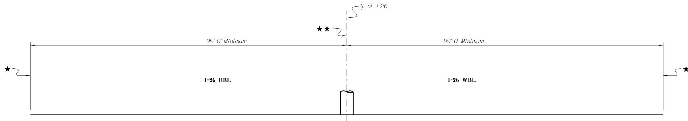
I-26 TYPICAL SECTION SHOWING HORIZONTAL CLEARANCE REQUIREMENTS UNDER NEW OVERPASSES
