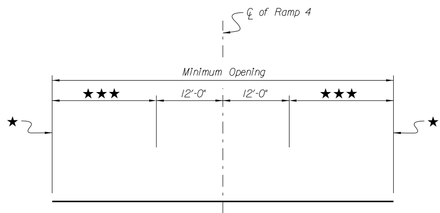
RAMP 4 TYPICAL SECTION SHOWING HORIZONTAL CLEARANCE REQUIREMENTS UNDER NEW OVERPASS
